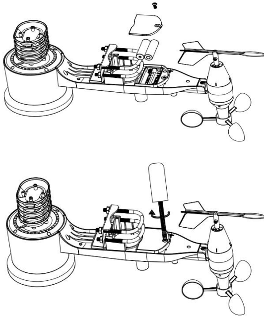
Figure 7: Battery installation diagram
